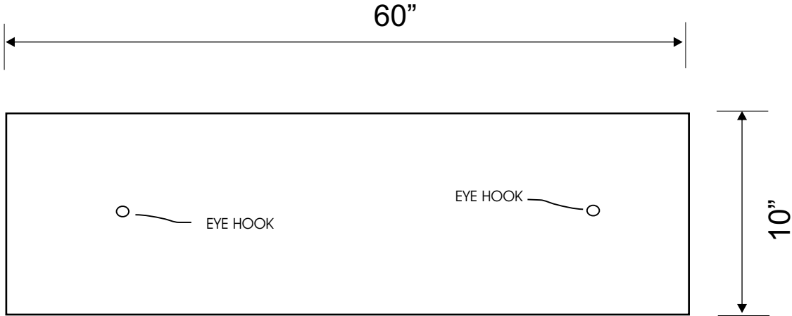
TOP VIEW
