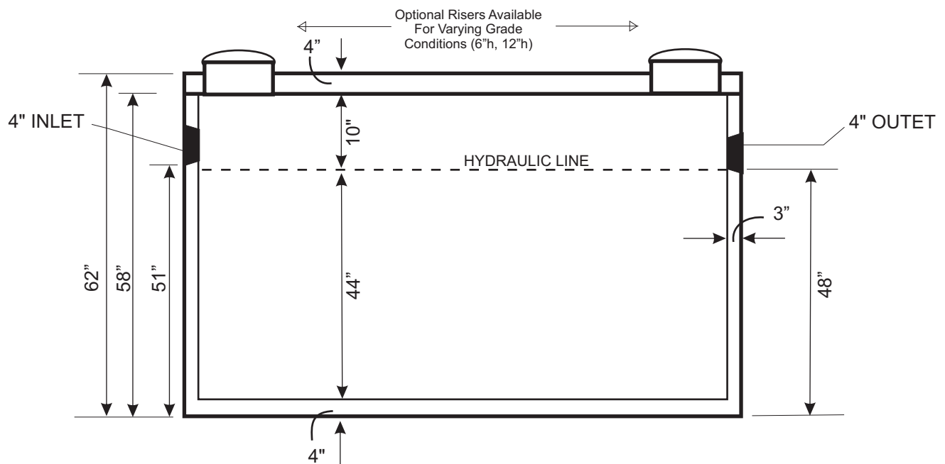
SECTION VIEW
